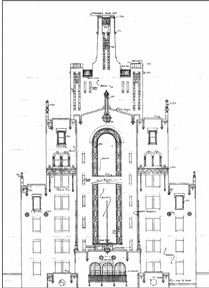
William Macy Stanton, Detail, South Elevation, James Madison Hotel , 1926, Atlantic City, New Jersey
